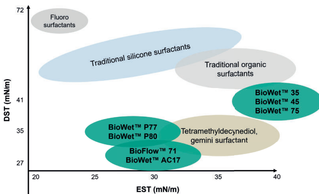
Surface tension of 1.0% additive in demineralised water:
